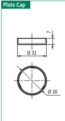
Plate Cap
