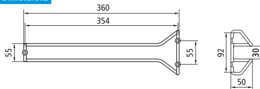
Long Version, Length 14-3/16" (360 mm)
