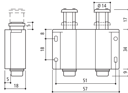
Dimensions Round Double Type
