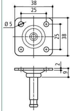
Swivel Plate
