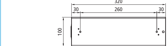
Short Version, Length 12-5/8" (320mm)
