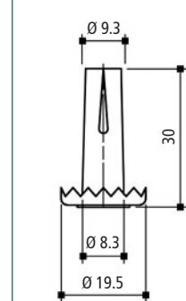
Metal Bushing
