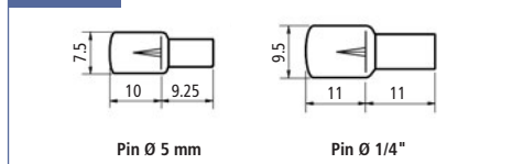
Spoon-Shape with Fin (anti-slip/slide) - Steel
