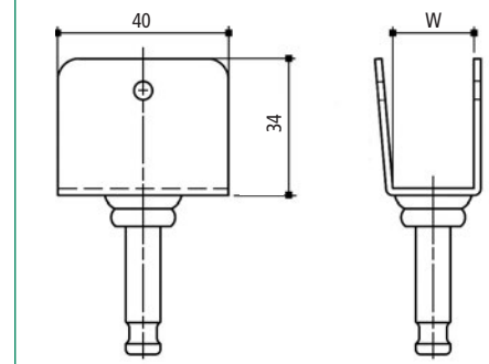
U-Bracket
