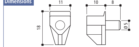
Plastic Shelf Support - with 5 mm steel pin
