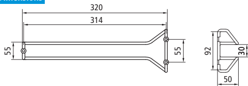
Short Version, Length 12-5/8" (320 mm)
