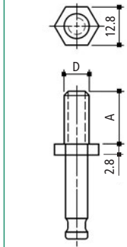
Threaded Stem
