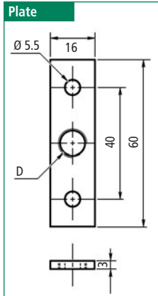
Plate
