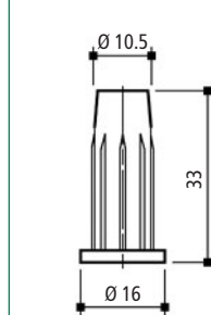
Nylon Bushing
