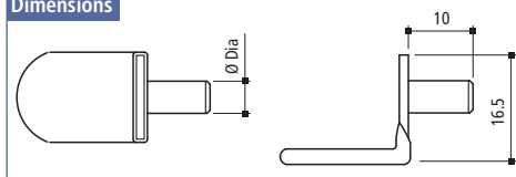
L-Shape - Steel with vinyl coating
