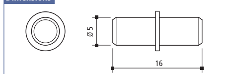
Pin type with Stop (Duplo) - Steel
